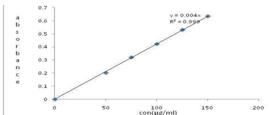
Fig 1: Standard calibration curve of Ranolazine in phosphate buffer pH 6.8
